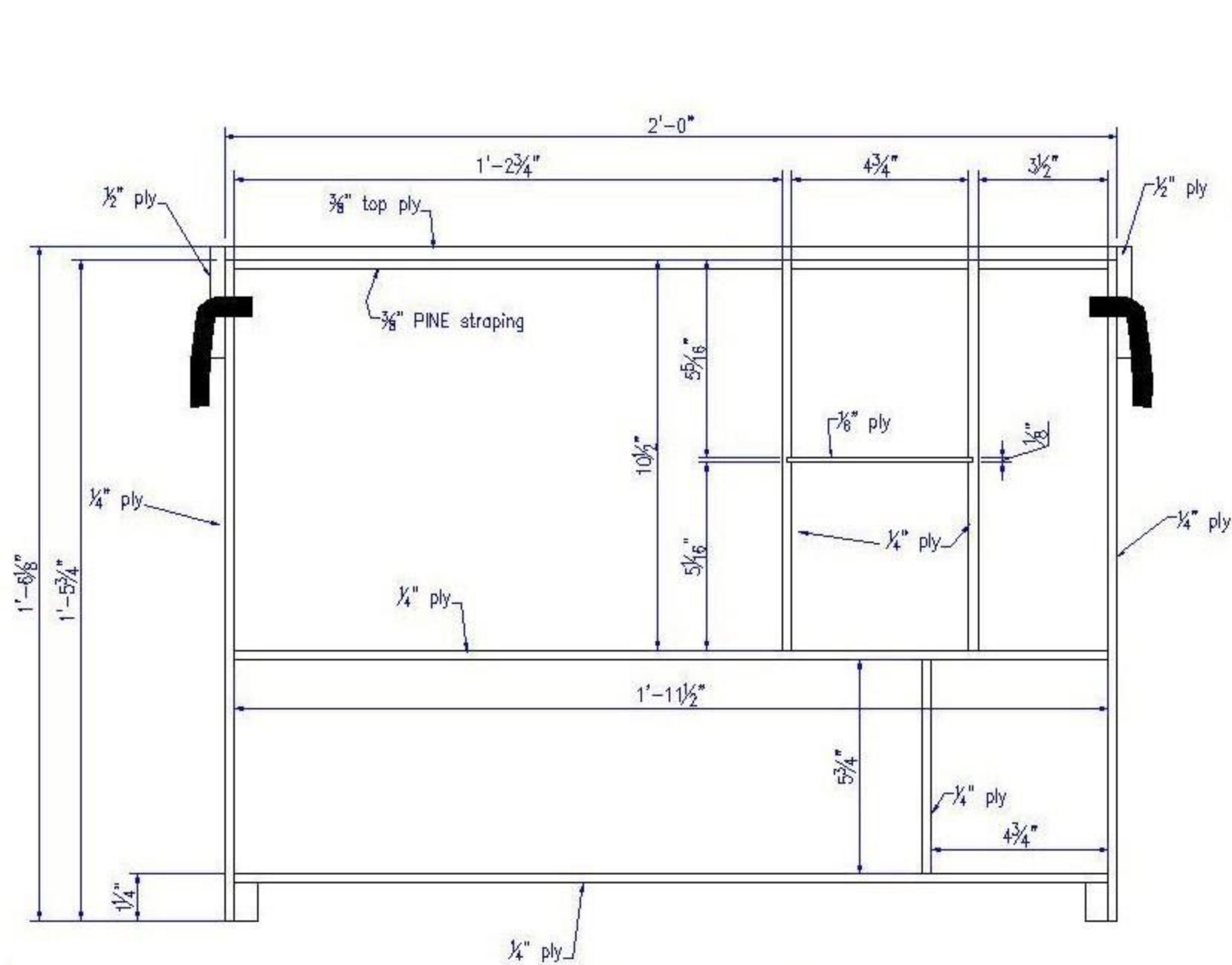
FRONT VIEW (DOORS OMITTED)
