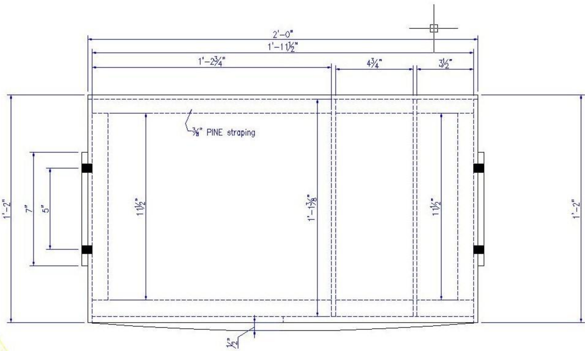
TOP VIEW
